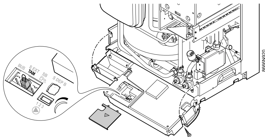
Module compact 2 circuits (EA 104) + Tubulure de raccordement (EA 106)
